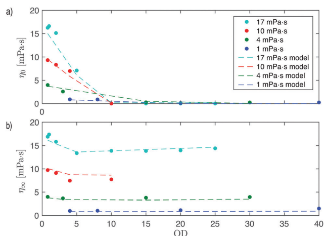
Fig. 6 Empirical model for Newtonian plateau values at low and high shear. Piecewise functions are used in the empirical model (dotted lines) to recover the viscosity values measured experimentally (solid circles) at (a) low shear ( \eta_0 ) and (b) high shear ( \eta_\infty ) for all bacterial concentrations (OD) tested.
