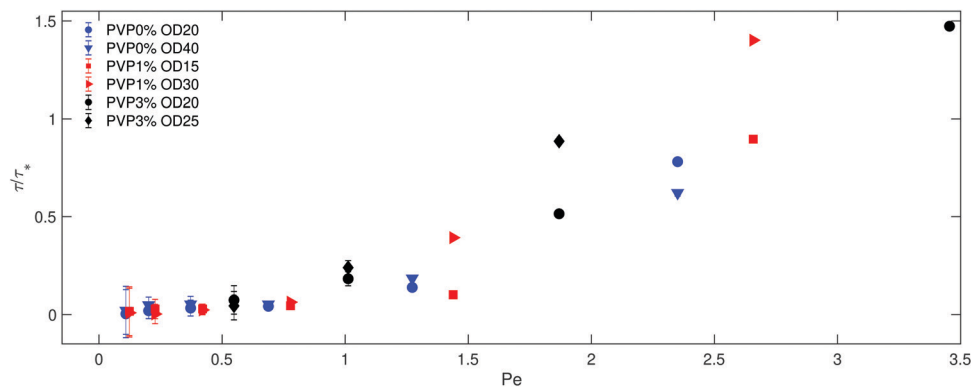
Fig. 8 Normalized stress \tau/\tau_* , where \tau_* = \eta_\infty D_r as a function of the Péclet number Pe = \dot{\gamma}/D_r . Blue circles: (OD = 20, \eta_s = 1 mPa s). Blue triangles: (OD = 40, \eta_s = 1 mPa s). Red squares: (OD = 15, \eta_s = 4 mPa s). Red triangles: (OD = 30, \eta_s = 4 mPa s). Black circles: (OD = 20, \eta_s = 14 mPa s). Black diamonds: (OD = 25, \eta_s = 14 mPa s).
