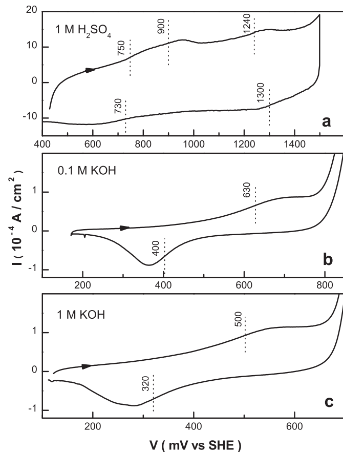
Fig. 2. Cyclic voltammograms for a cleaved (001) \text{Sr}_2\text{IrO}_4 single crystal surfaces (from top to bottom: dV/dt = 50, 10, 14 \text{ mV/s} , \text{pH} = 0.3, 13, 14 ). The dotted lines indicate the steepest slope location of the redox peaks.
