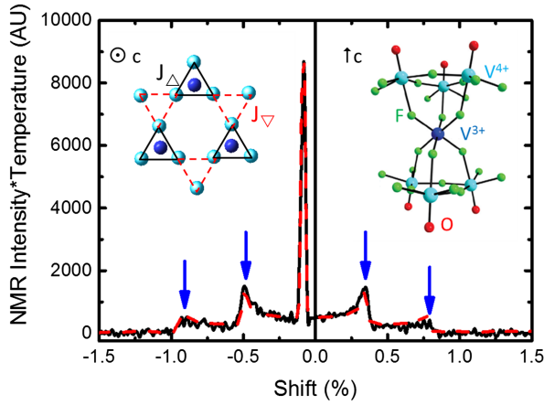
FIG. 1. ^{17}\text{O} NMR spectrum of DQVOF at 300 K and H_0 = 7.5 T (black line) and the simulation of the powder spectrum (red dashed line). The blue arrows point to the quadrupolar singularities. The shift reference is \nu_0 = {}^{17}\gamma/2\pi \times H_0 = 43.288 MHz ( {}^{17}\gamma/2\pi = 5.772 MHz/T). Left inset: Top view of the magnetic lattice with the \text{V}^{4+} (light blue spheres) forming the breathing kagome lattice and the interlayer \text{V}^{3+} (dark blue spheres). Right inset: Local environments of the vanadium ions.
