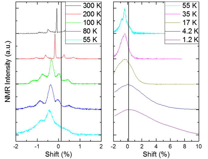
FIG. 2. ^{17}\text{O} NMR spectra over a selected range of temperatures. The spectra are normalized to their maximum value. The black vertical lines show the reference for the spin shift.
