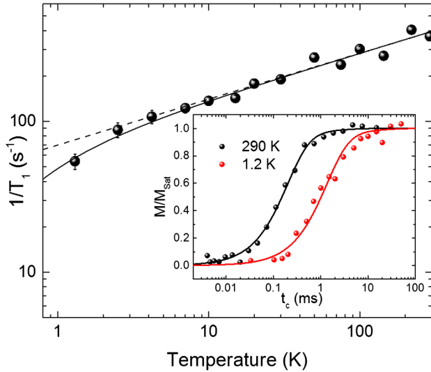
FIG. 4. Thermal evolution of 1/T_1 . The solid line is a fit as explained in the text. The dashed line shows the T^{0.3} variation. Inset: Recovery curves at 290 and 1.2 K.
