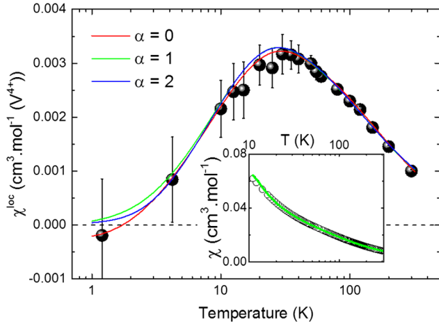
FIG. 3. Local NMR susceptibility of the kagome layers \chi^{\text{loc}} . The lines are fits to A\chi_{\text{kago}}^{\text{th}} + C (see the text). Inset: SQUID macroscopic susceptibility (circles) and fit to a combination of \chi_{\text{kago}}^{\text{th}} ( \alpha = 1 ) and a paramagnetic contribution from the V^{3+} (line) [24].
